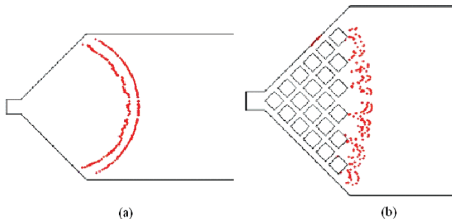
Figure 4. Particle trace snapshot at a distance of 17 mm from the injection edge. Channel dimensions are 3.5 \text{ mm} \times 2 \text{ mm} \times 100 \mu\text{m} . The average flow velocity used was 1.5 \text{ mm/s} in the main section of the channel. The end piece in part b uses 200\text{-}\mu\text{m} square microstructures.
